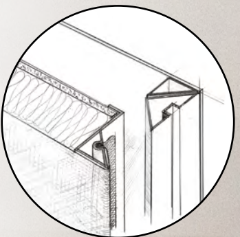
PANNELLO ACUSTICO ACOUSTIC PANEL
